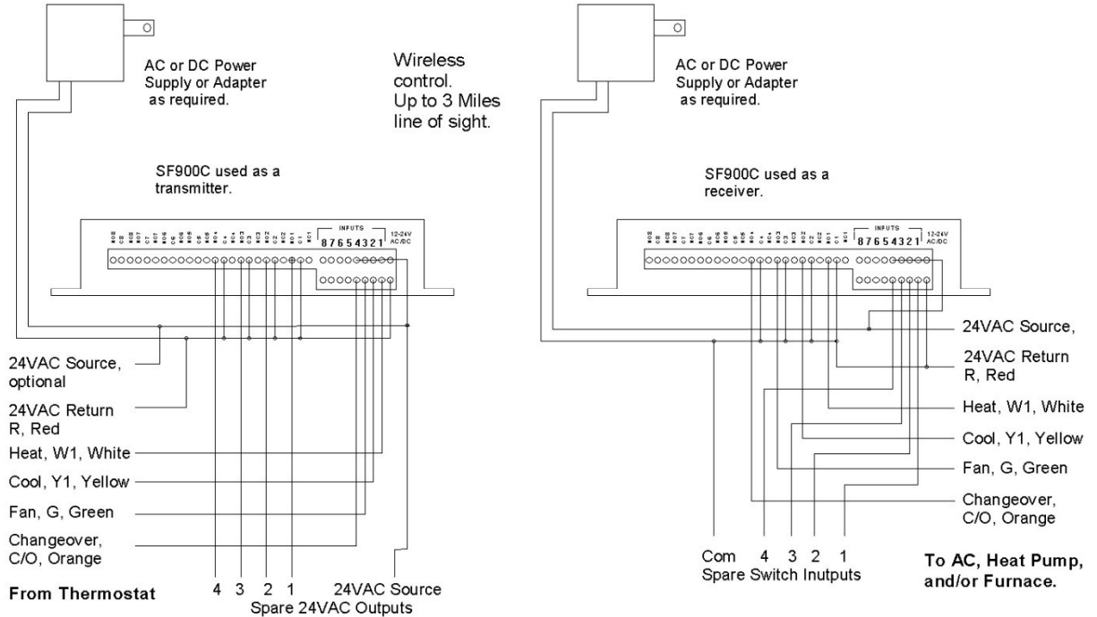
Application Circuit - Thermostat to HVAC
